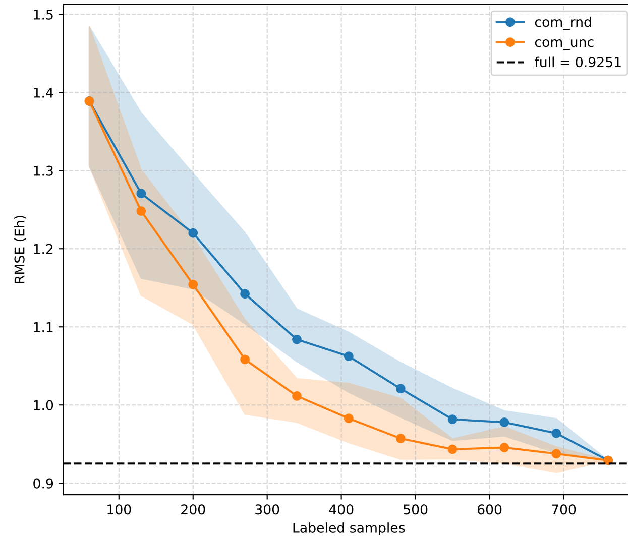
RMSE (Eh)
