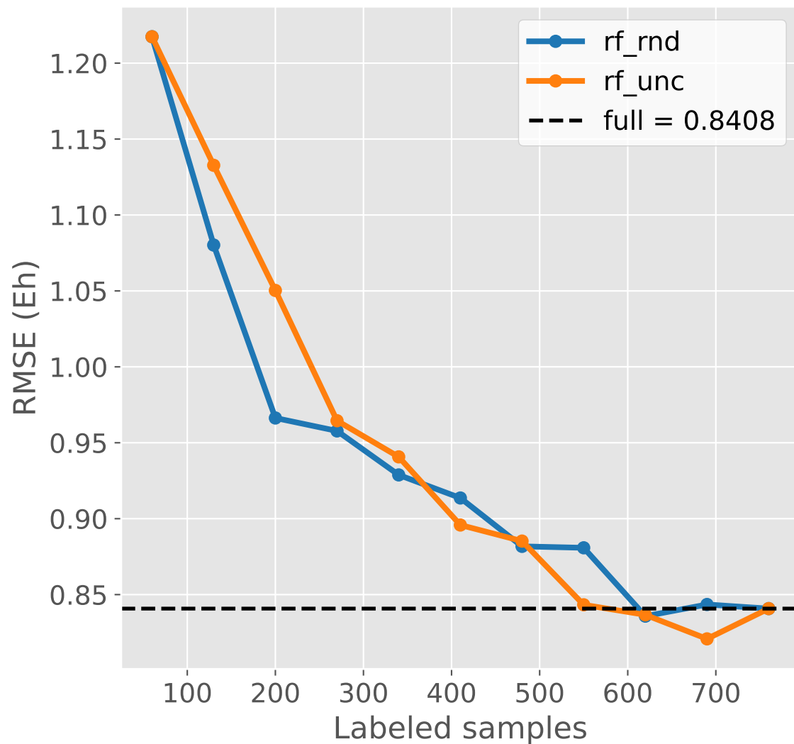
RMSE (Eh)
