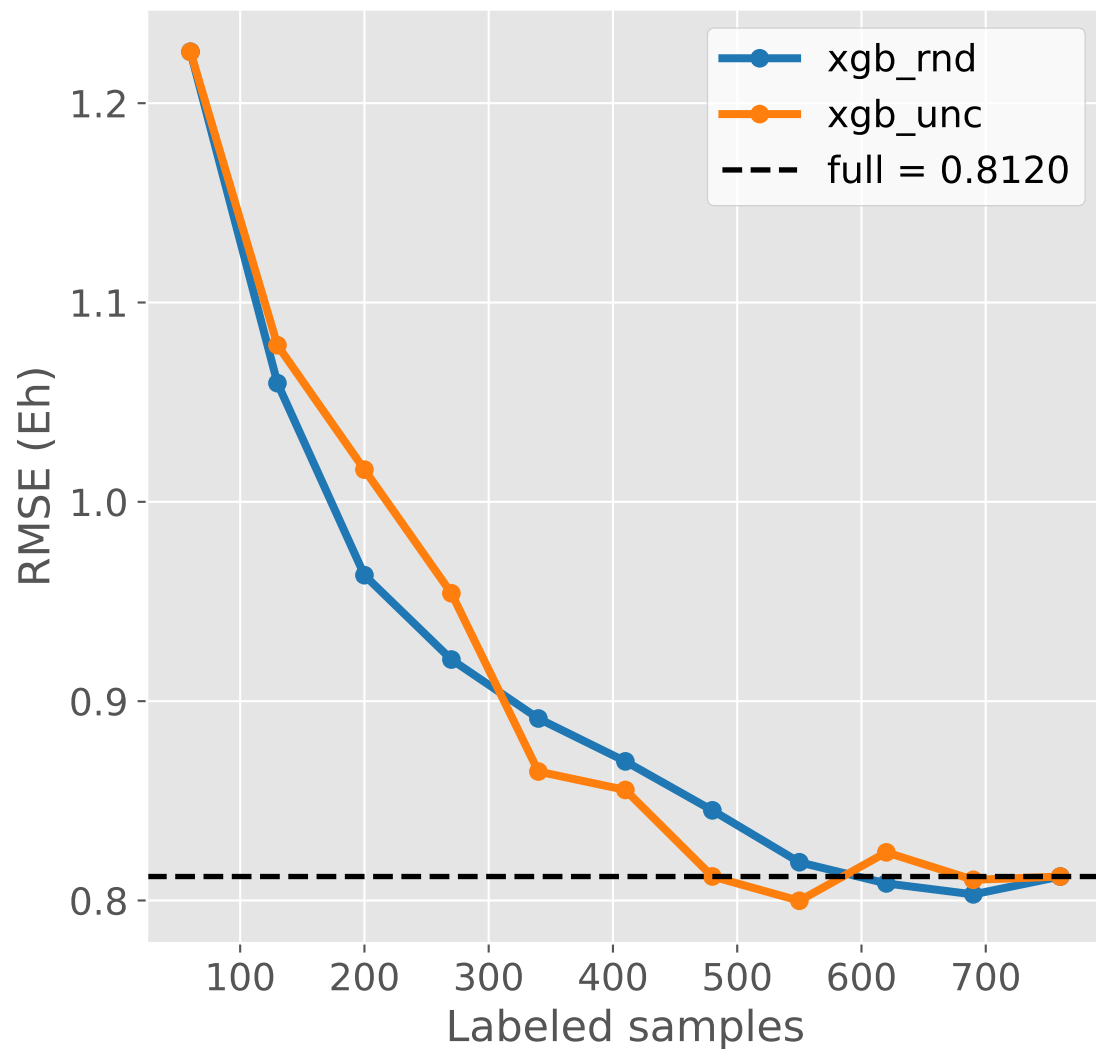
RMSE (Eh)
