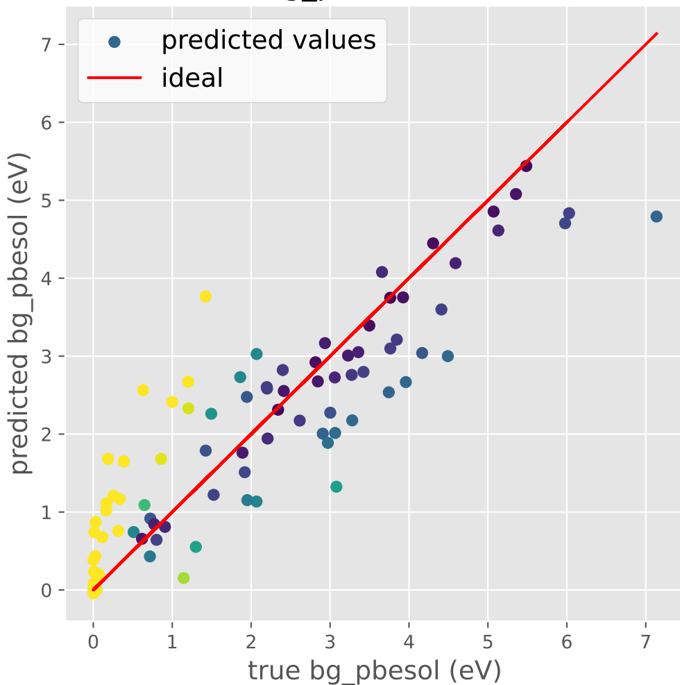
Committee prediction plot bg_pbesol (eV)
