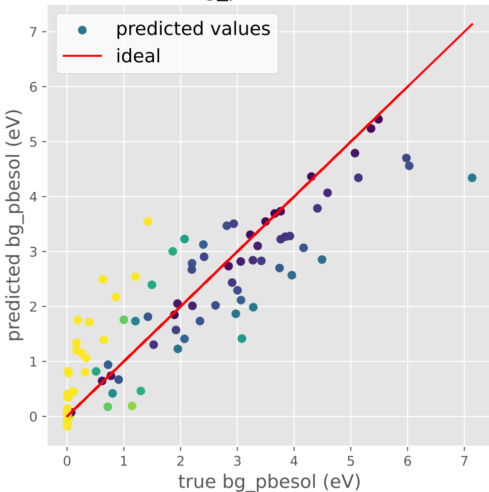
KR prediction plot bg_pbesol (eV)
