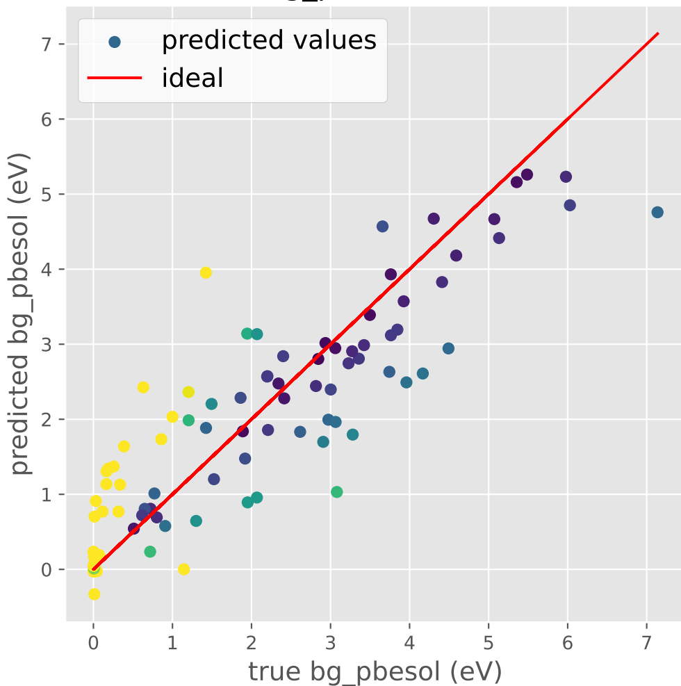
XGB prediction plot bg_pbesol (eV)
