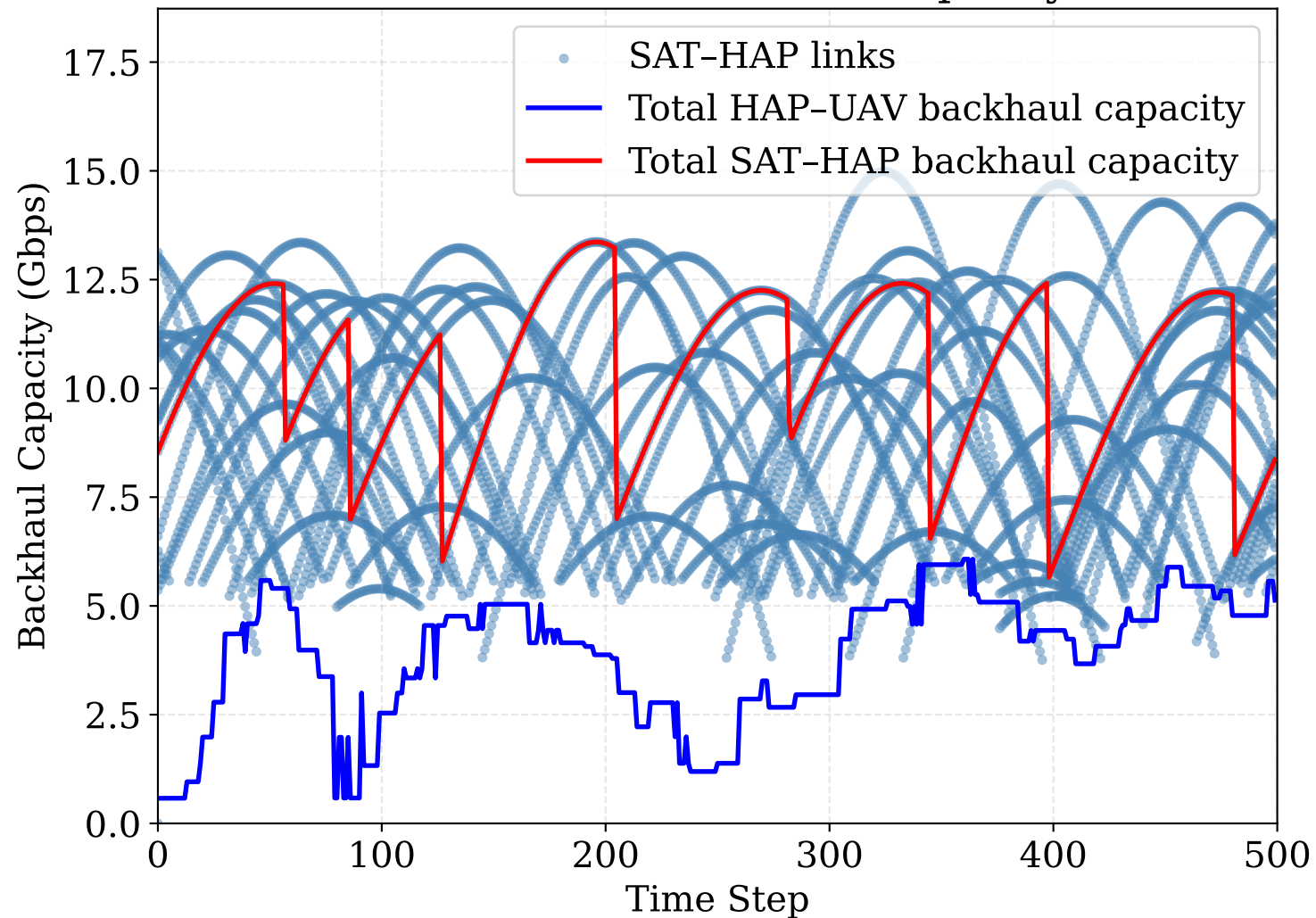
SAT-HAP and HAP-UAV Backhaul Capacity Over Time
