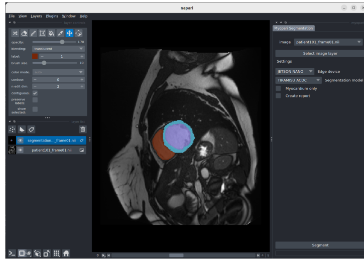
Fig. 2. Myopari Napari plugin for automated CMR analysis. This simple workflow enables automated segmentation, biomarker extraction, 3D rendering, and structured reporting. Users only need to select the hardware and AI model; the plugin then executes the full analysis pipeline with one click.
