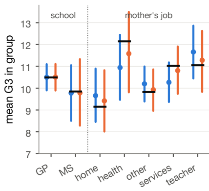
(c) group means: observed vs predictive 95%
