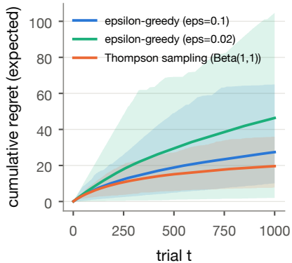
A: well separated p = 0.599, 0.500, 0.401
