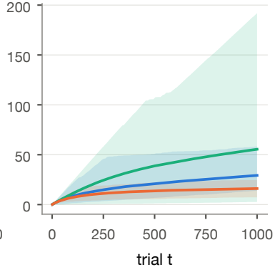
C: hard task, one expert p = 0.525, 0.332, 0.289
