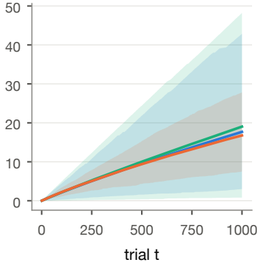
B: close abilities p = 0.525, 0.500, 0.475
