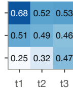
C: learned (CTS)
