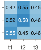
B: learned (CTS)
