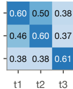
A: learned (CTS)
