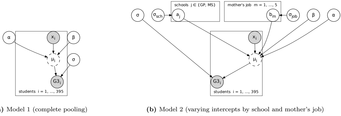
Figure 1: Plate diagrams. x_i : standardised predictors; \mu_i = \alpha + x_i^\top \beta (+ a_j + b_m in Model 2); G3_i \sim \mathcal{N}(\mu_i, \sigma) .
