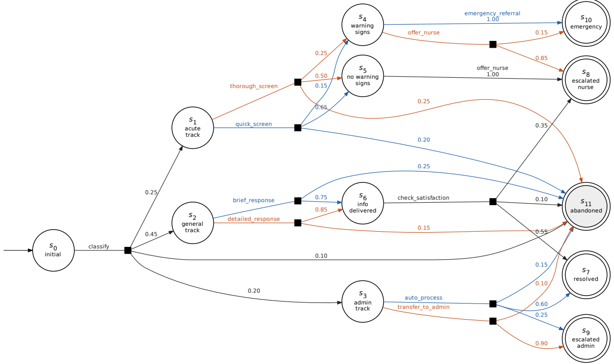
Figure 6: The HealthLine MDP. Circles: states; double circles: terminal states; black squares: probabilistic branching points of the actions; edge labels: action names and transition probabilities. In the decision states s_1-s_4 the two actions are drawn in blue and orange, so each probability can be traced to its action.
