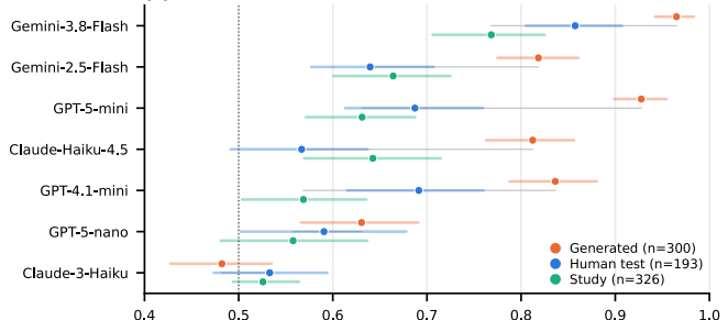
(a) Per-model AUROC
