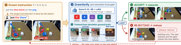
Figure 1: The pilot validator as a pre-execution trust gate (DrawVerify pilot, 2026): a LoRA-adapted VLM trained on simulator ground truth judges the marked image and caption; ACCEPT executes, REJECT asks the user to redraw.
