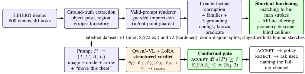
Figure 2: Method sketch (referenced from Section 3.2). Top : simulator-grounded data generation (green = new). Bottom : the validator generates a structured verdict and a reason; a conformal threshold yields an execute/ask decision.
