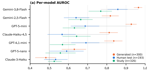
Figure 3: Pilot evidence (referenced from Section 4): AUROC of seven API validators on generated prompts, the human test split and the in-the-loop study (95% bootstrap intervals). Generated prompts rank models like human sketches do but inflate absolute scores unevenly, motivating H1 and H3.
