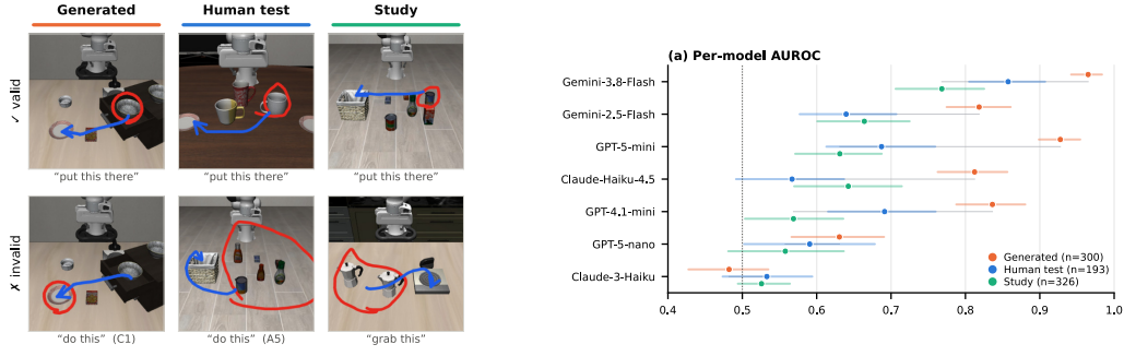
Figure 2: Pilot evidence for the evaluation plan (DrawVLA-Verify pilot, 2026). Left : three evaluation sources, one valid (top) and one invalid (bottom) prompt each: generated prompts with a known failure mode (C1: circle on the plate, arrow from the bowl), held-out human sketches (A5: one circle encloses several bottles), and in-the-loop study sketches (both moka pots circled, so “grab this” has no unique referent). Right : AUROC of seven API validators on the three sources (95% bootstrap intervals): generated prompts rank models like human sketches do but inflate absolute scores unevenly, motivating H2 and H4.
