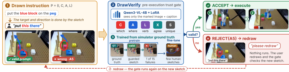
Figure 1: The pilot validator as a pre-execution trust gate (DrawVLA-Verify pilot, 2026): a LoRA-adapted VLM trained on simulator ground truth judges the marked image and caption; ACCEPT executes, REJECT asks the user to redraw.
