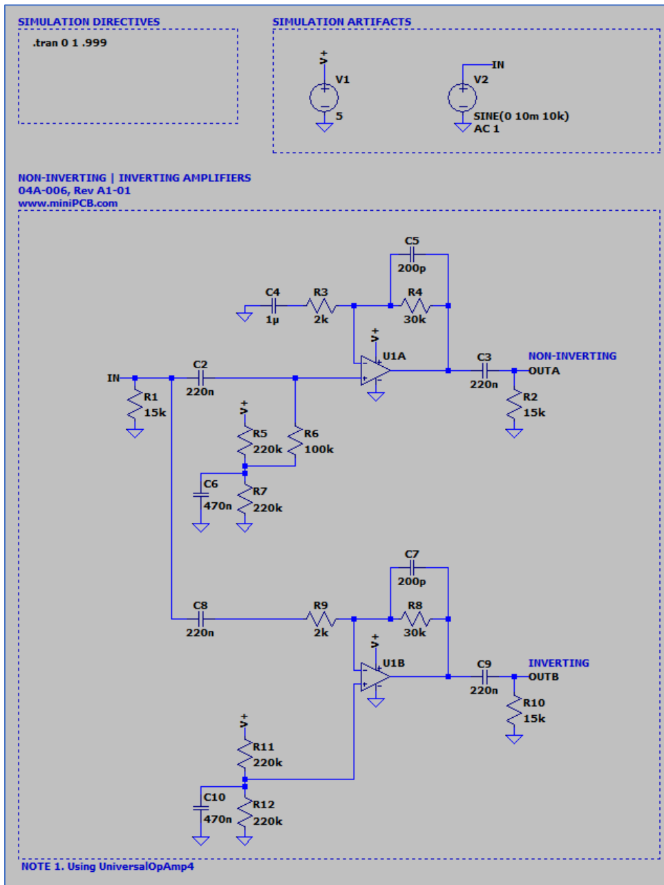
Figure 2 - LTspice Simulation, Schematic
