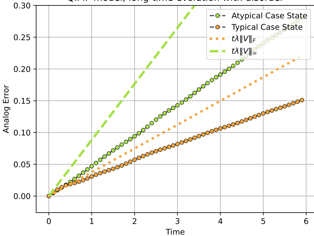
QIMF model, long-time evolution with disorder
