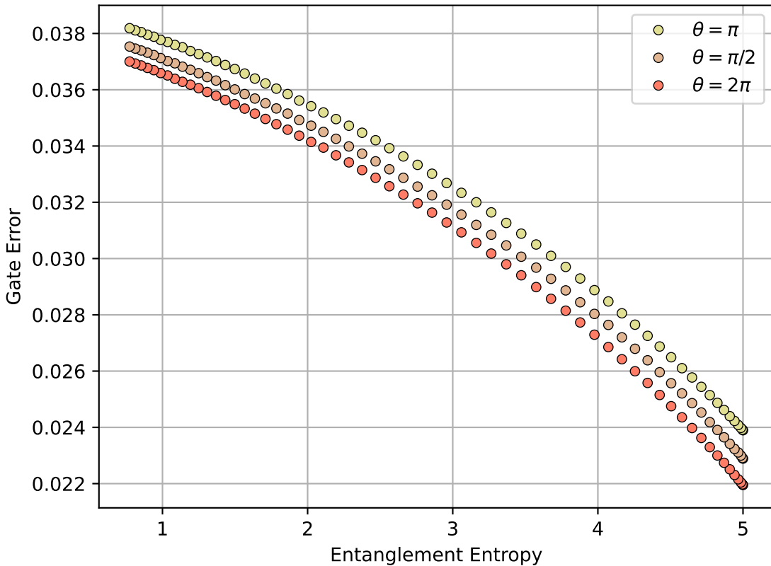
Quantum Dot, Robust Control Pulses
