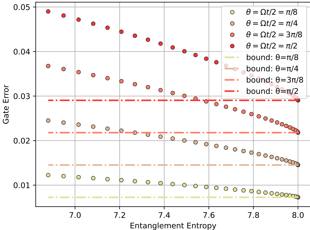
Quantum Dot, 2-qubit Gate
