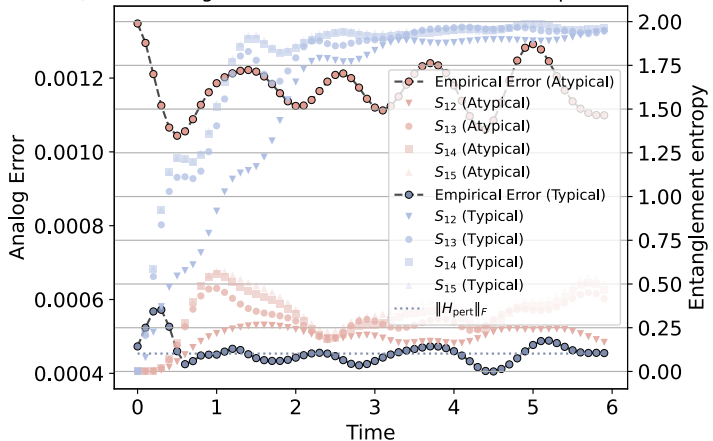
B QIMF, one segment evolution with disorder & imperfections
