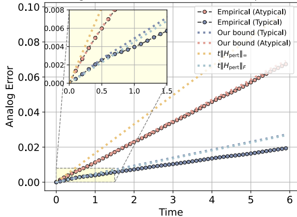
A QIMF, long-time evolution with disorder & imperfections
