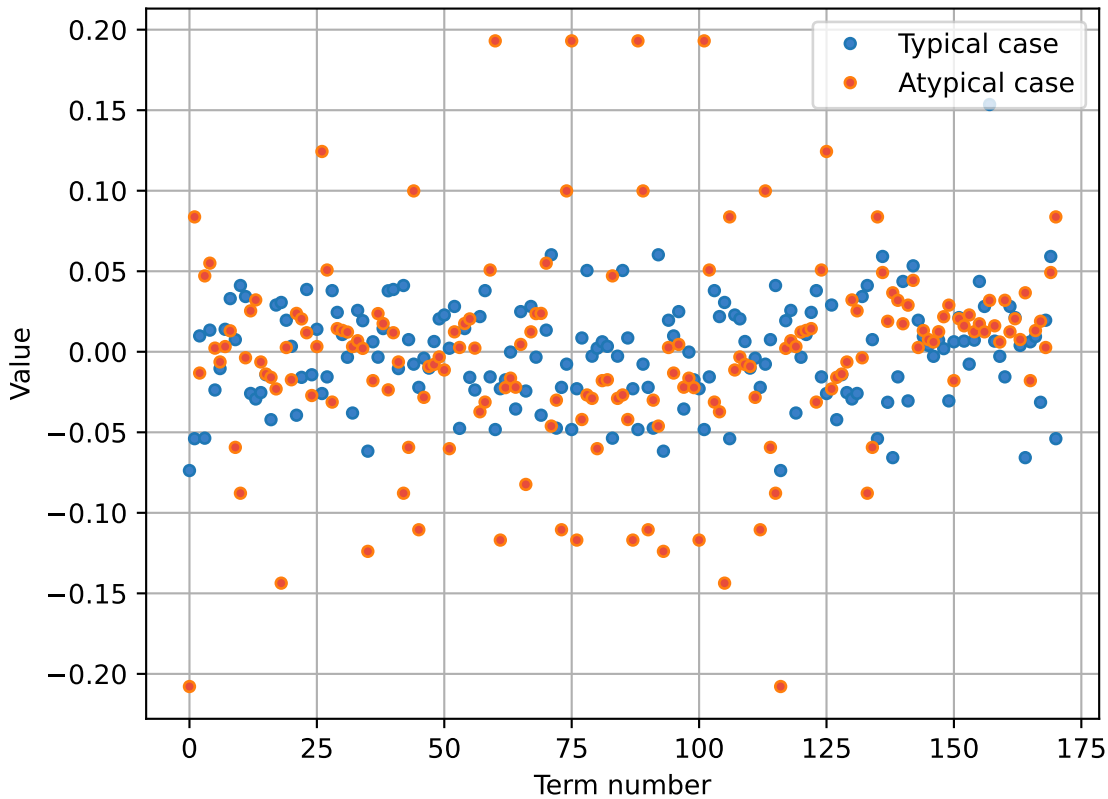
QIMF model, long-time evolution
