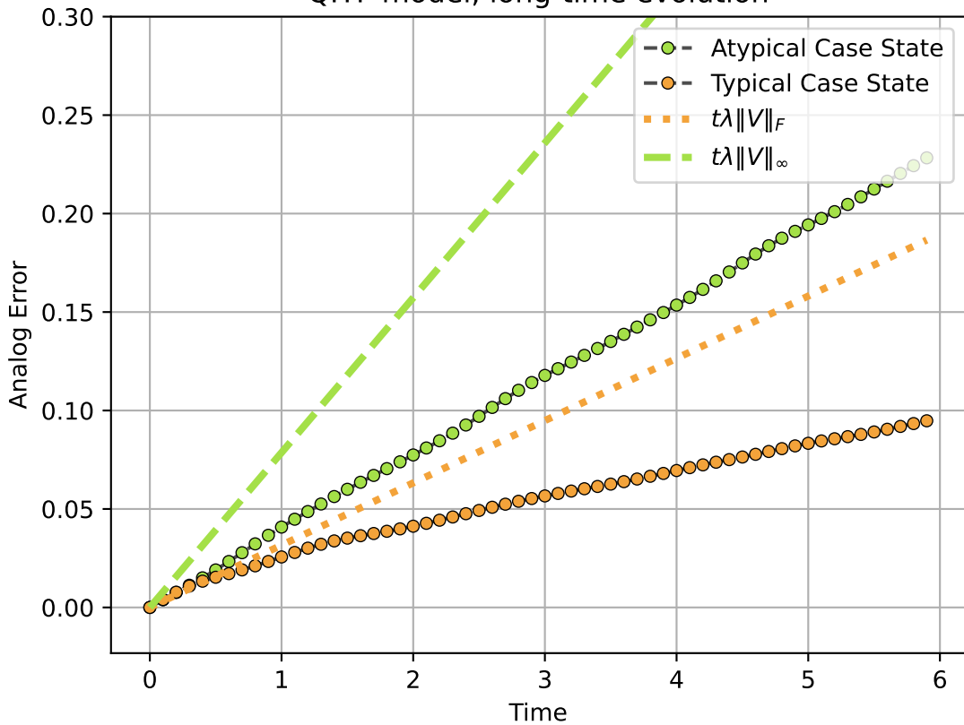
QITF model, long-time evolution
