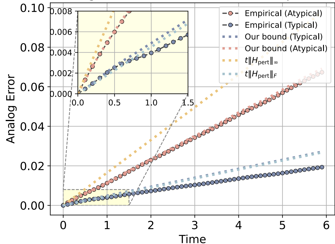
QIMF, long-time evolution with disorder &amp; imperfections
