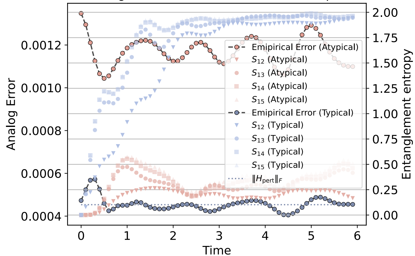
QIMF, one segment evolution with disorder &amp; imperfections
