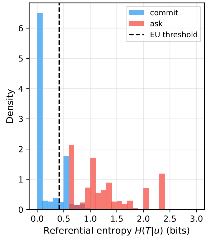
(a) Entropy by action
