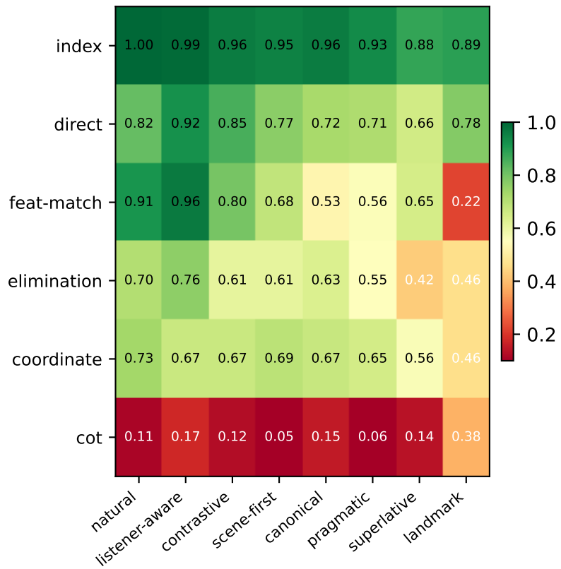
(c) CPA heatmap ( N = 8 , none)
