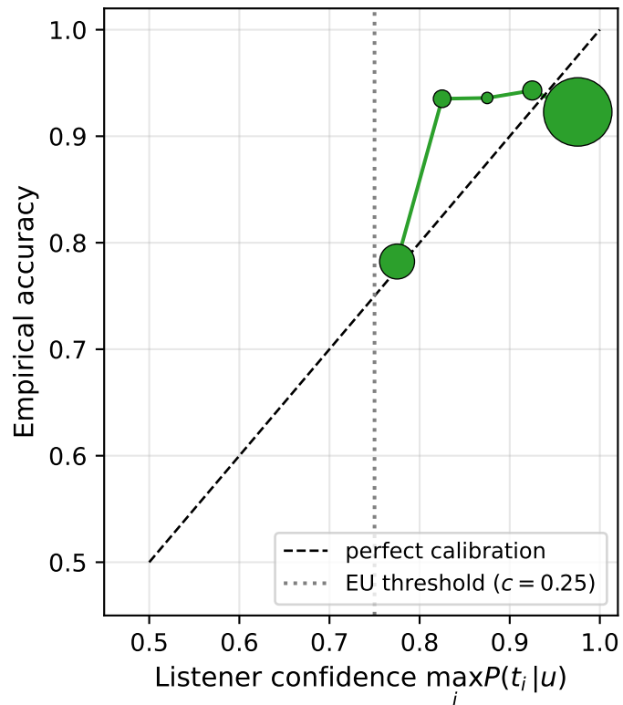
(b) Calibration on committed scenes
