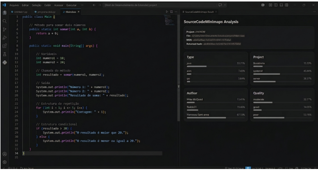
Figure 4: Visual Studio Code extension displaying the Web-View interface with minimap visualization and prediction groups.
