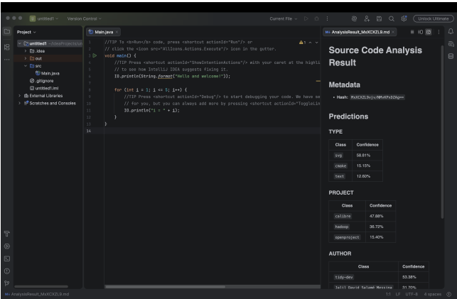
Figure 3: IntelliJ IDEA plugin showing Markdown-based feedback in split-screen generated from source code analysis.
