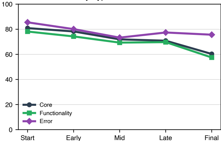
Test Pass Rates by Type
