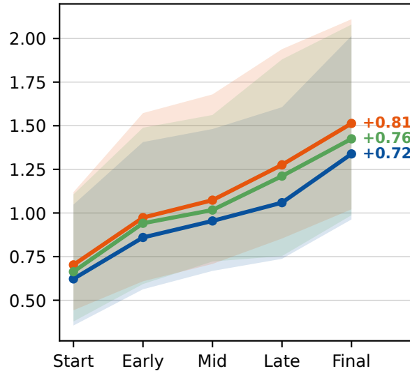
$ / Checkpoint
