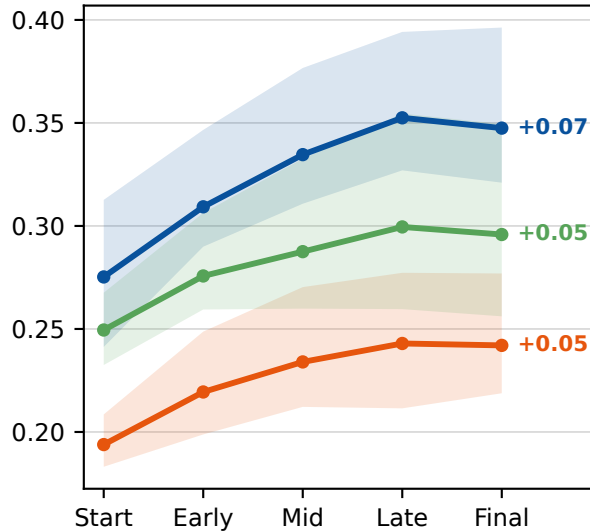
Verbosity
