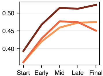
Anthropic Verbosity
