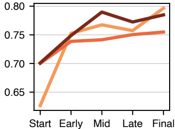
Anthropic Erosion
