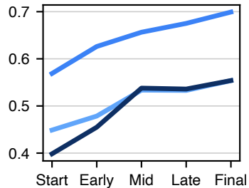
OpenAI Erosion
