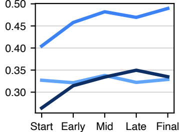
OpenAI Verbosity
