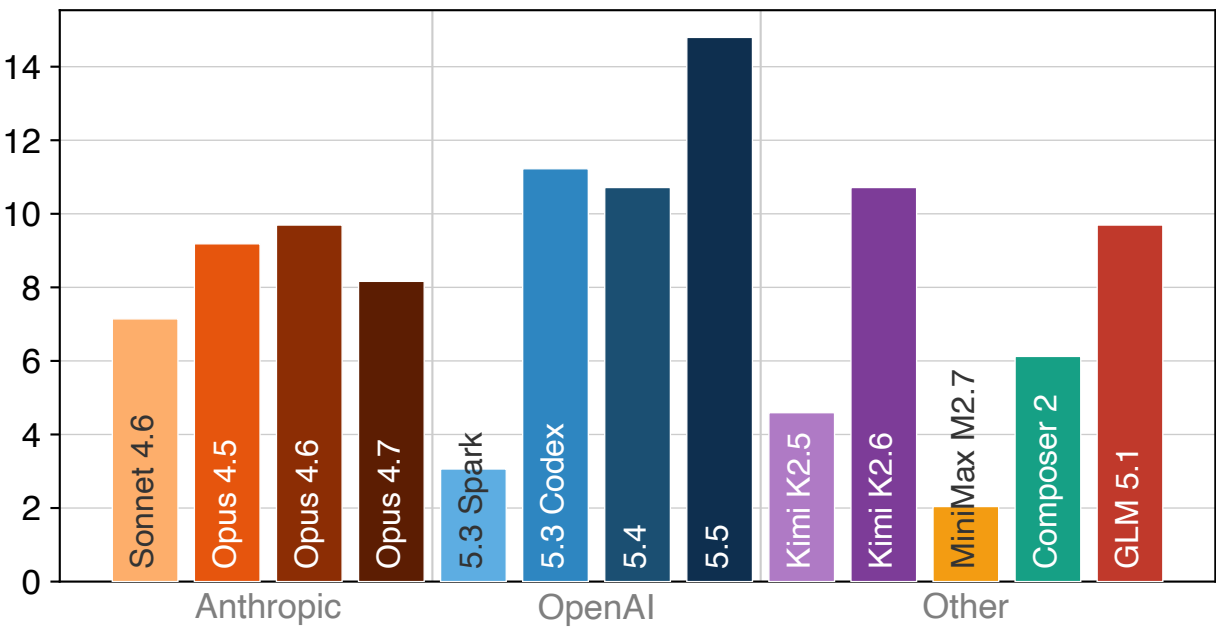
Strict Solve Rate (%)
