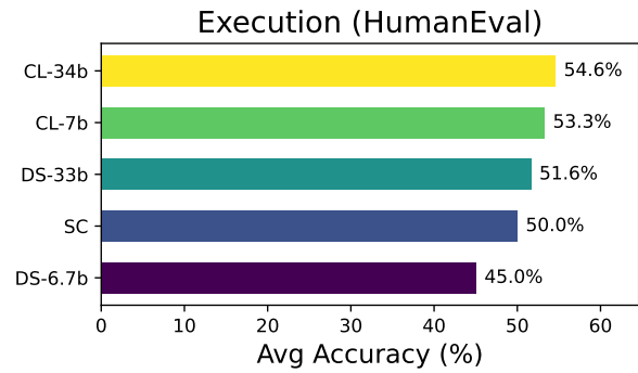
(b) Execution (HumanEval)
