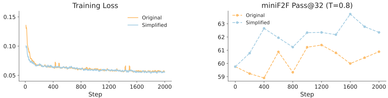
Figure 4.5: Training loss (left) and miniF2F score (right) after SFT on simplified vs. original proofs.
