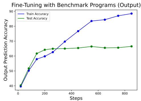
Figure 3.6: Improvements and Limits of CRUXEVAL Performance after Fine-Tuning
