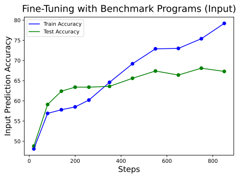
Figure 3.6: Improvements and Limits of CRUXEVAL Performance after Fine-Tuning
