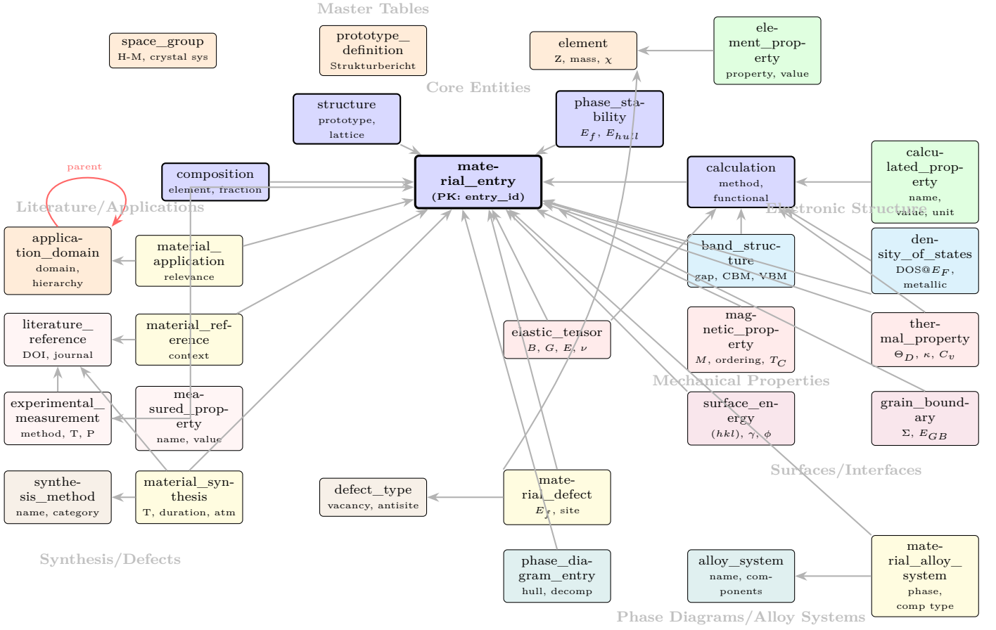
Figure 3: ER diagram of the 30-table validation database. Centered on material_entry , core tables such as composition , structure , and phase_stability are directly connected by FKs, while calculated properties, electronic structure, and mechanical properties, surface energy, and related data are accessed through two or more hops. Gray arrows indicate FK relationships, and the red arrow indicates a self-referencing FK (the hierarchical structure of application_domain ). Yellow tables are N:M junction tables.
