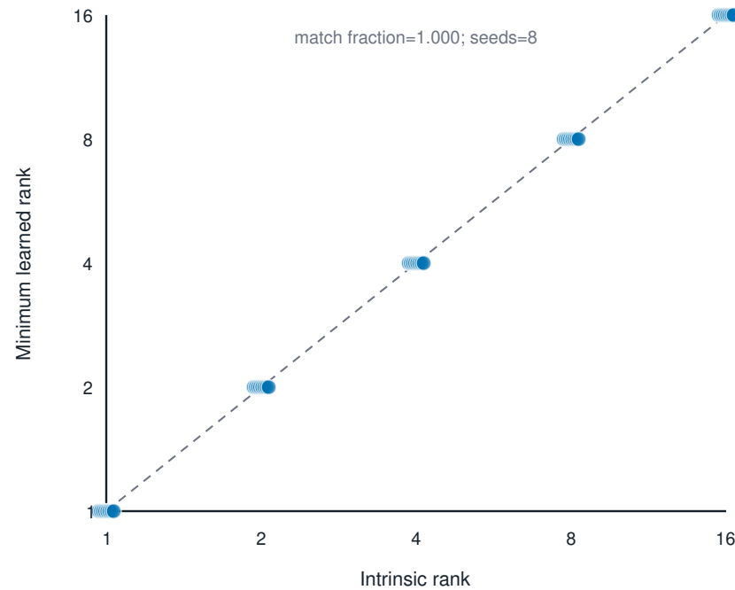
B Learned control-rank scaling
