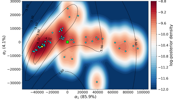
Figure 2: The PMPD plot corresponding to full-bandwidth data centered around the sample mean (green square) for Experiment 1a. The posterior samples are shown as cyan circles, and the ground truth model is shown as a yellow star. The black dashed lines show the log-misfit contours. The percent variation of the samples along each principal component ( \alpha_1 and \alpha_2 ) are shown in parenthesis on the axes.
