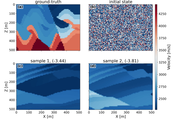
Figure 5: Experiment 2 plots: (a) The ground truth model for Experiment 2. (b) An example of the pure noise initial state. (c,d) Two (out of 50) samples generated by DPS-based inversion. The log-misfit of the posterior samples are shown in parenthesis next to the sample number.
