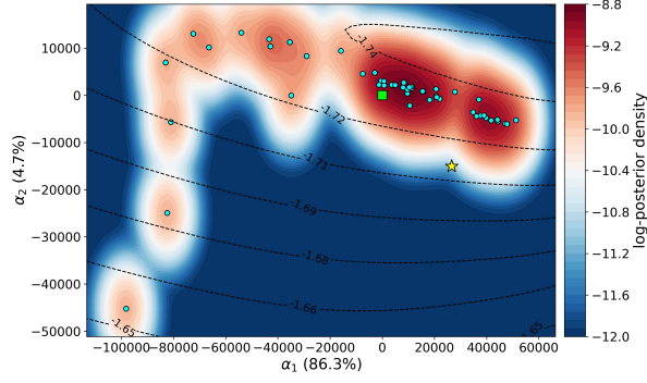
Figure 4: The PMPD plot corresponding to data lacking sub 5 Hz frequencies centered around the sample mean (green square) for Experiment 1b. The posterior samples are shown as cyan circles, and the ground truth model is a yellow star. The black dashed lines show the log-misfit contours. The percent variation of the samples along each principal component ( \alpha_1 and \alpha_2 ) are shown in parenthesis on the axes.
