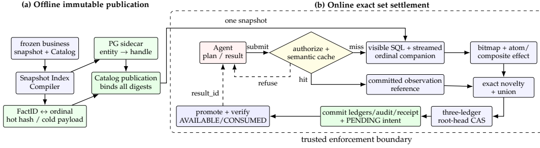
Fig. 1. (a) Offline publication fixes ordinals and the Merkle-radix Outcome set; (b) online exact settlement, promotion, and replay.
