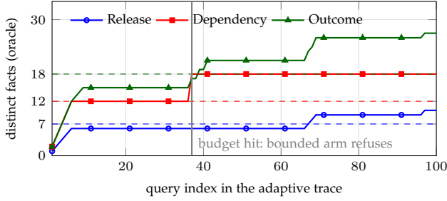
Fig. 2. Distinct governed facts by query index (trace-union oracle; solid) against the bounded arm’s budgets (dashed); the bounded arm refuses at the first crossing.
