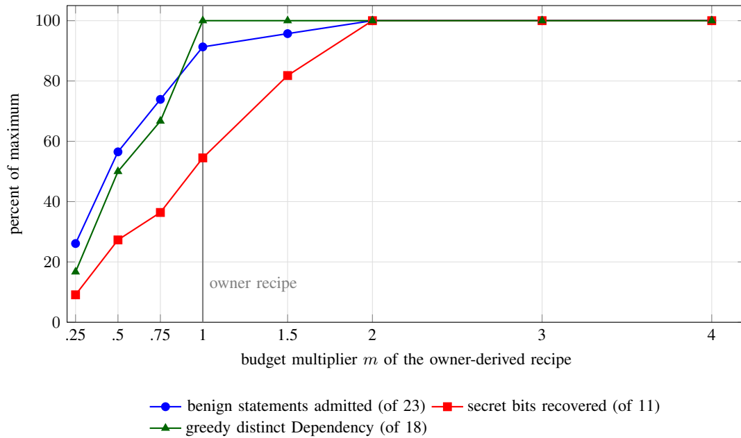
Fig. 1. Benign statement admission versus adversarial extraction as the owner recipe is scaled by m (scenario simulation: admission arithmetic over the frozen corpora’s closed-form footprints at eight multipliers; not executed, and not a bound on the deployed ledger). Executed points: benign 1 \times replays to 21/23 (pilot: 22/23, first refusal q26) and 2 \times / 4 \times all; adversary owner tier 6 bits and greedy 18, loosened 11 bits (pilots realized these tables).
