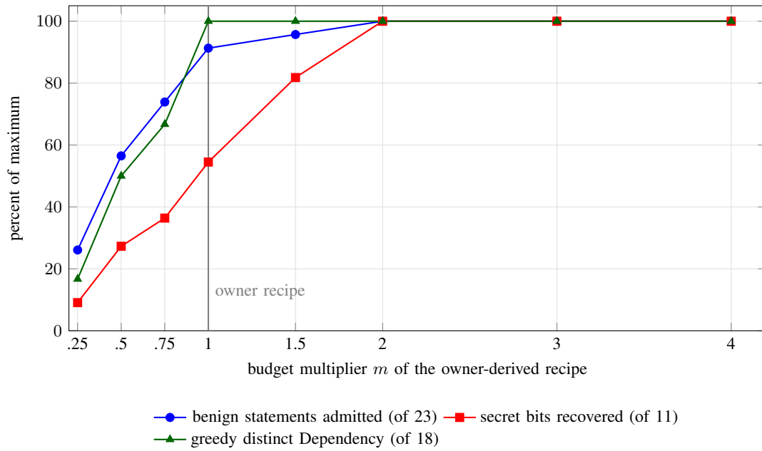
Fig. 1. Benign statement admission versus adversarial extraction as the owner recipe is scaled by m (scenario simulation: admission arithmetic over the frozen corpora’s closed-form footprints at eight multipliers; not executed, and not a bound on the deployed ledger). Executed points: benign 1 \times replays to 21/23 (pilot: 22/23, first refusal q26) and 2 \times / 4 \times all; adversary owner tier 6 bits and greedy 18, loosened 11 bits (pilots realized these tables).
