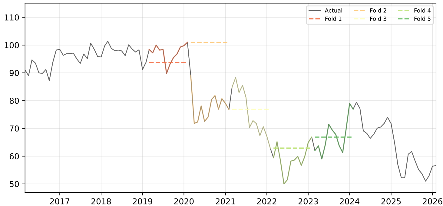
UMCSENT | NRMSE h=1: 0.078 h=12: 0.115
