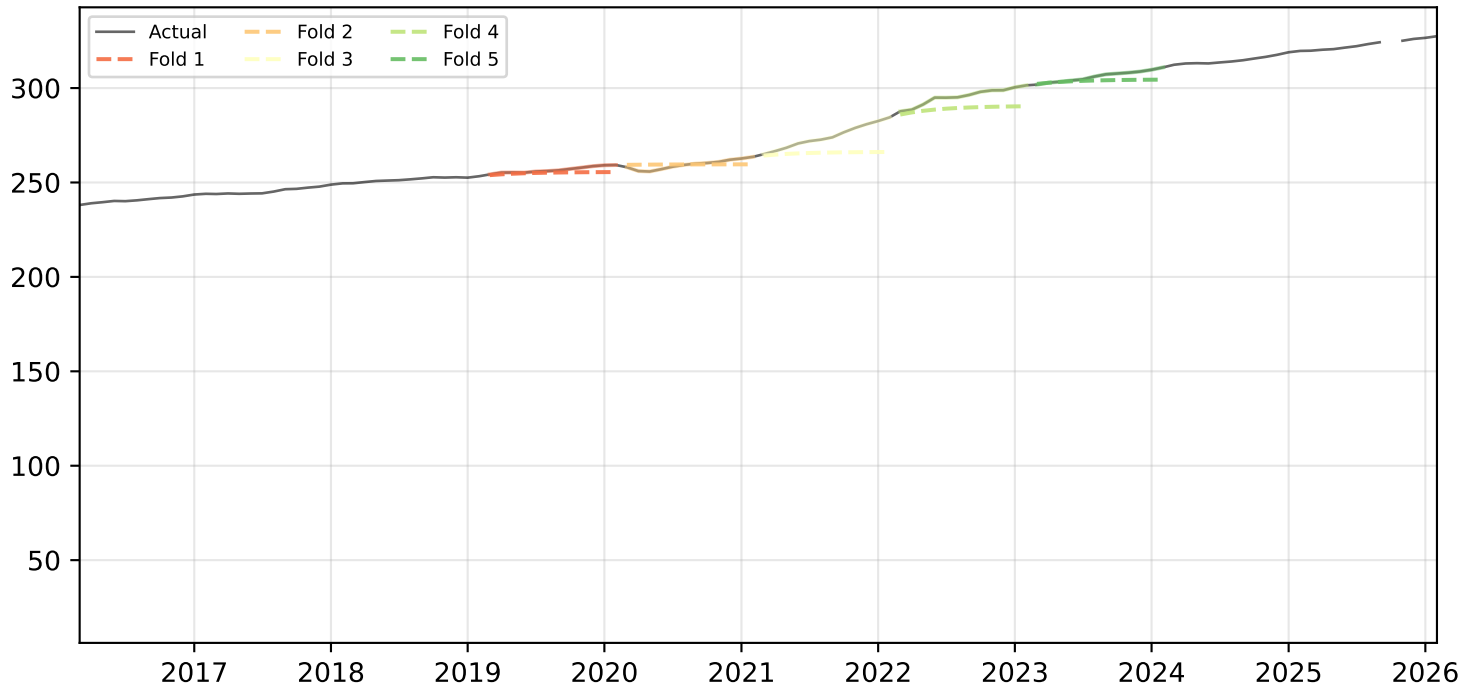
PAYEMS | NRMSE h=1: 0.006 h=12: 0.048
