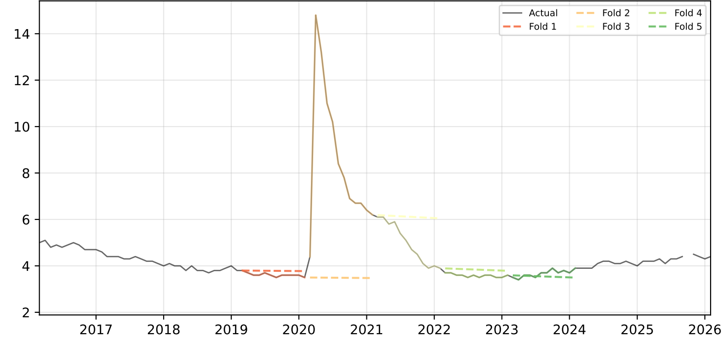
UNRATE | NRMSE h=1: 0.045 h=12: 0.281
