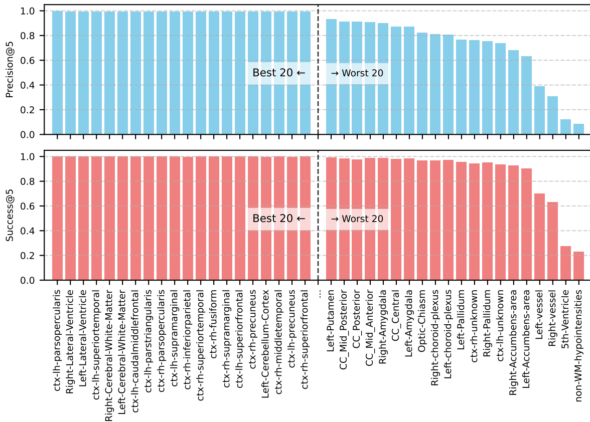
Top 20 Best & Worst Structures by Precision
