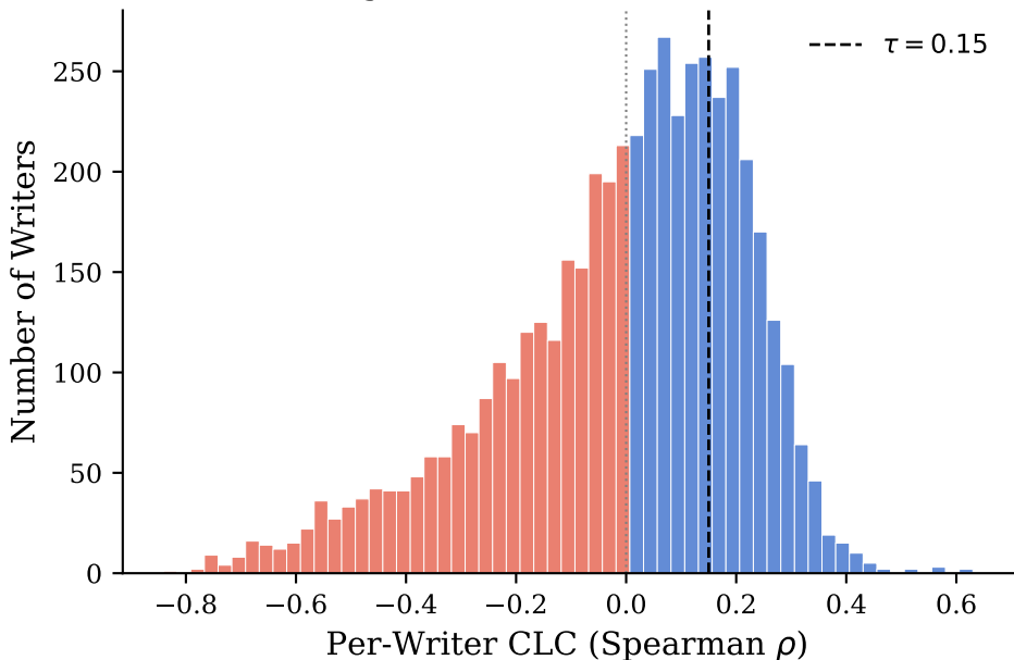
Per-Writer Cognitive-Load Correlation Distribution
