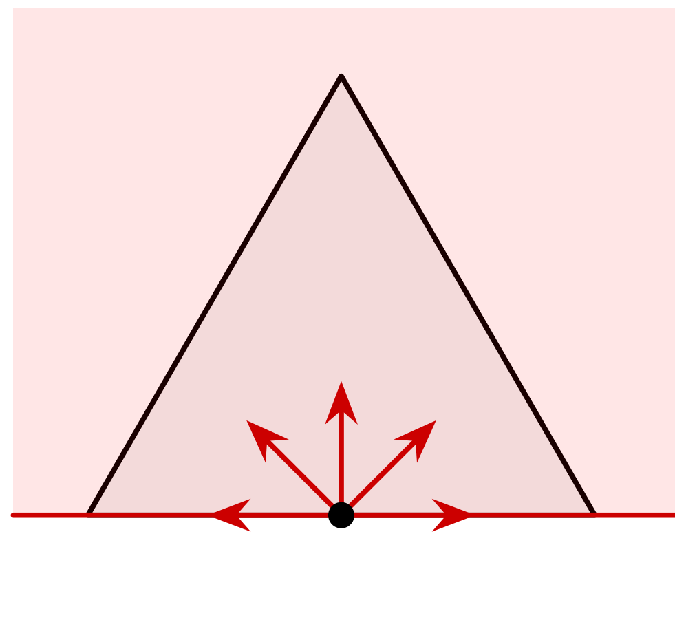
辺 x_3 = 0 h_3 \geq 0 \ (h \in L)
