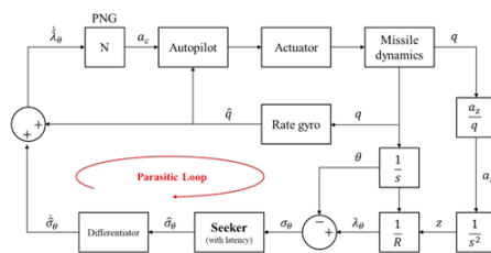
(b) Strapdown Seeker
