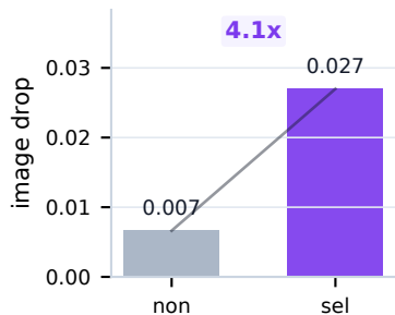
Image mass drop G-H
