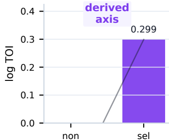
Log TOI gap H-G
