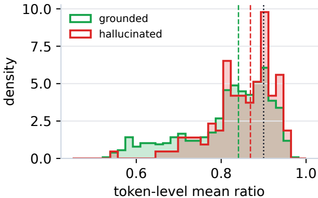
Object-token T/(T + I)
