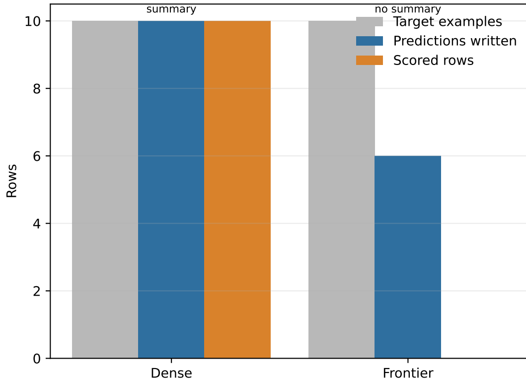
Artifact completion
