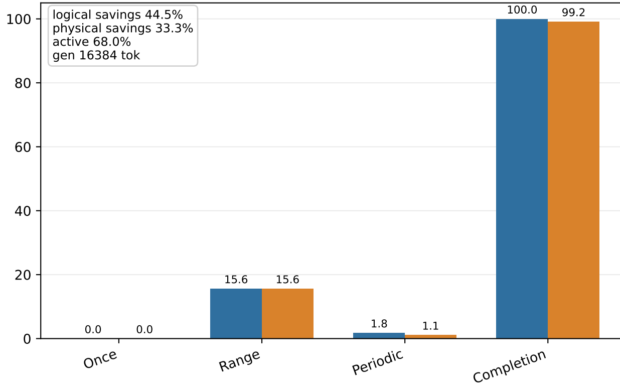
SGT short
