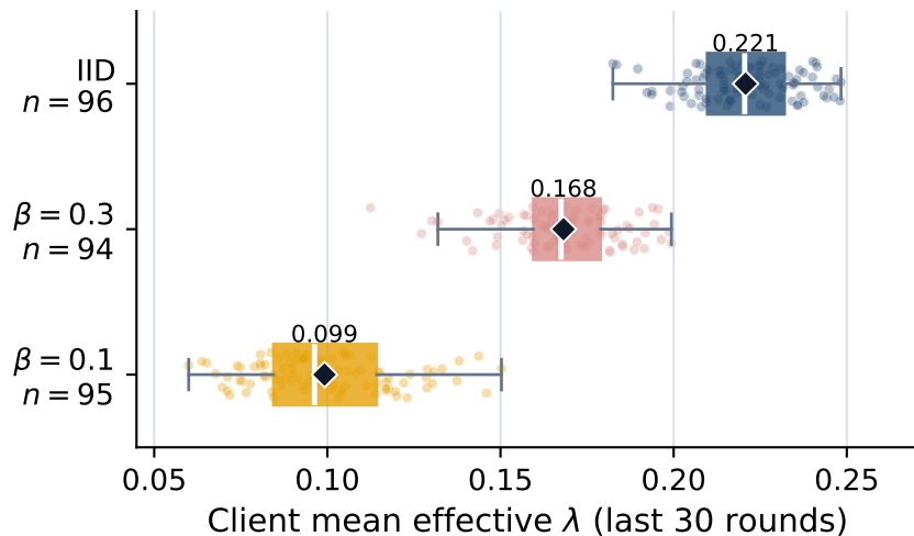
CIFAR-100
