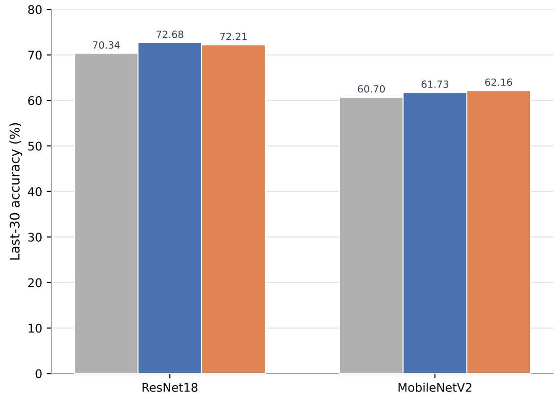
CIFAR-100
