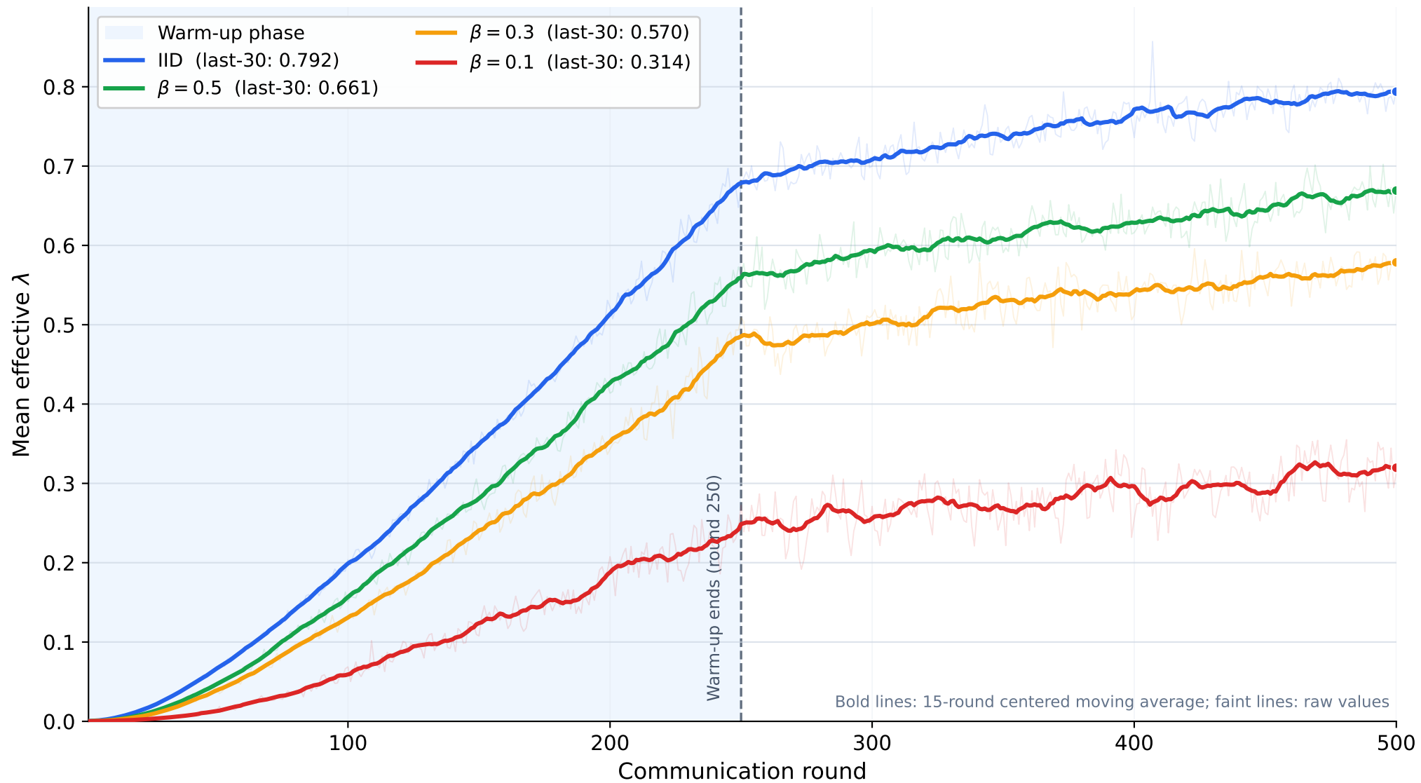
CIFAR-100: Round-wise Mean Effective \lambda
