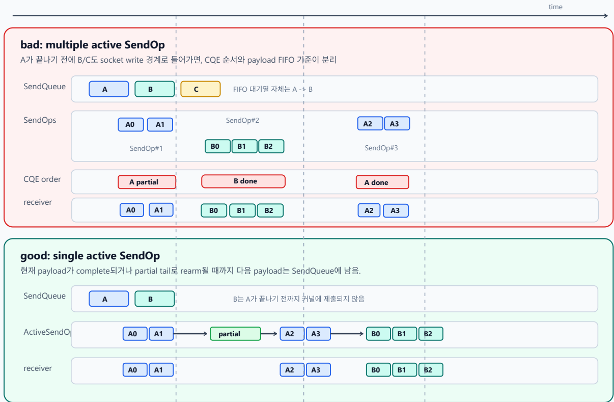
fig servercore sendop order timeline
