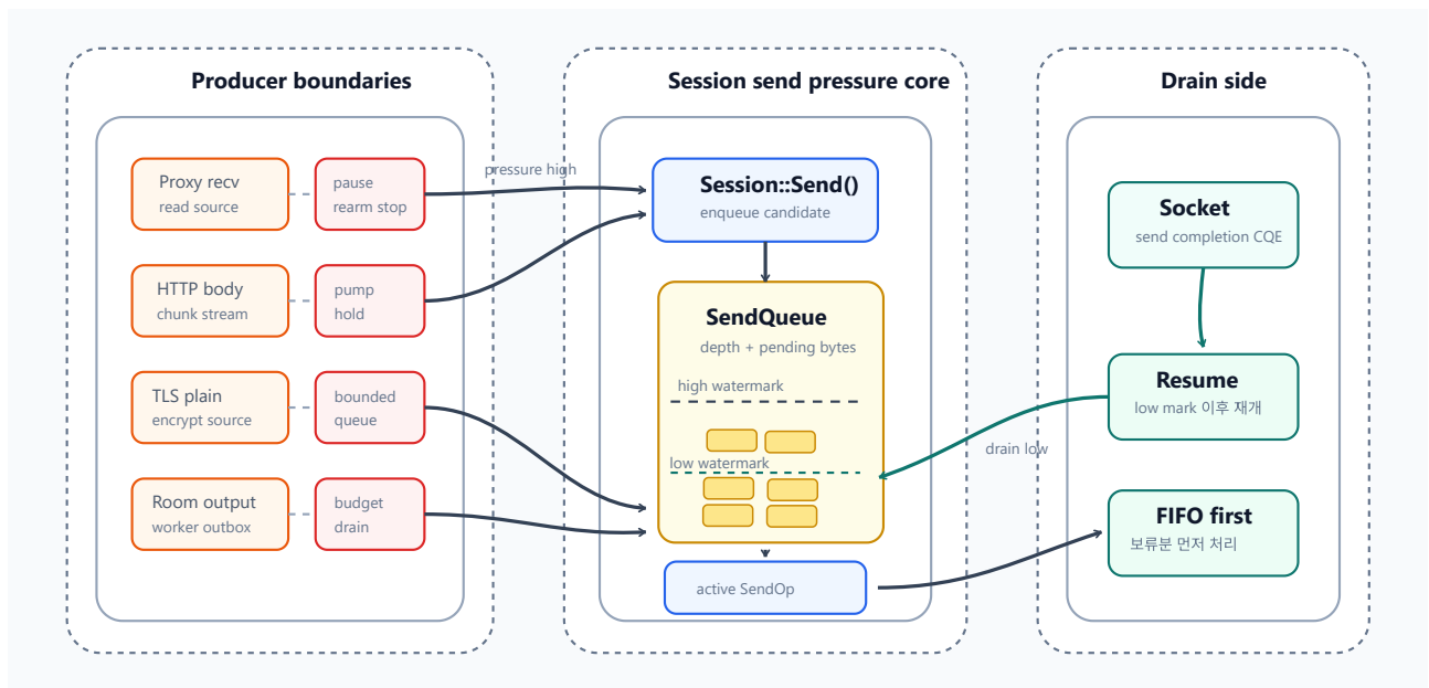
fig servercore backpressure
