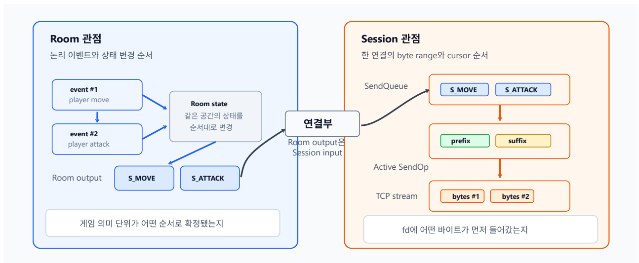
fig servercore ordering layers
